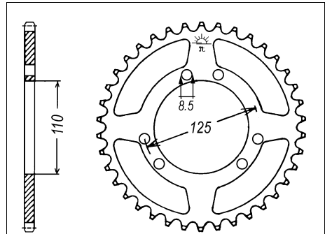
Chain 420
