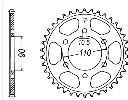
Chain 630
