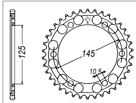
Chain 525
