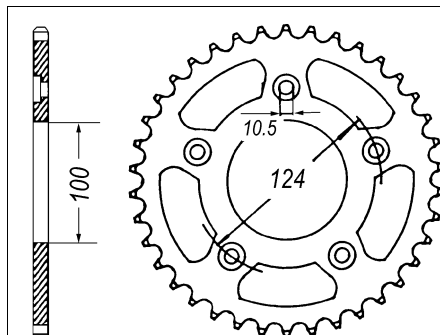
Chain 525
