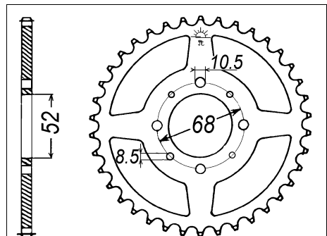
Chain 428
