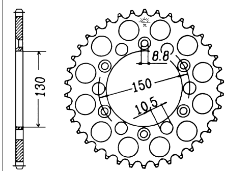
JTR 251/2
