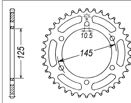
Chain 520
