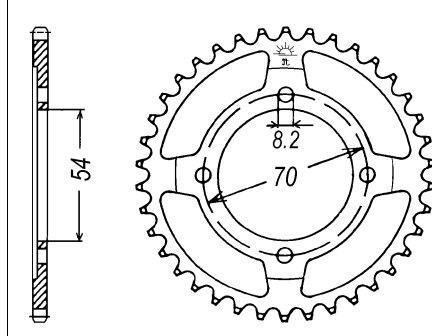
Chain 428
