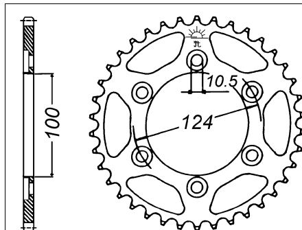
Chain 520
