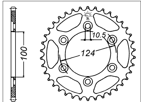
Chain 525
