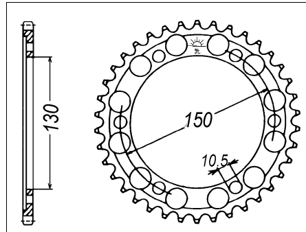
Chain 532
