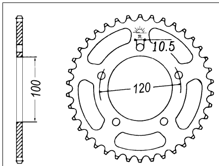
Chain 520
