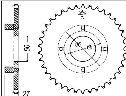
Chain 420
