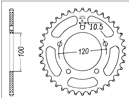
Chain 525
