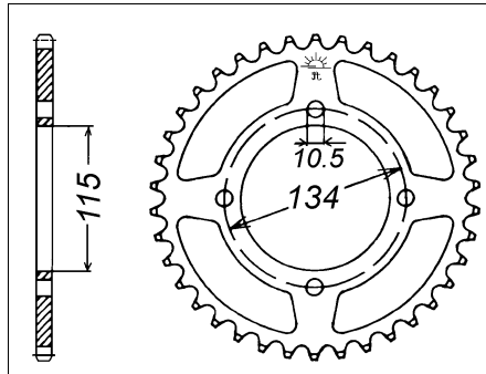
Chain 520
